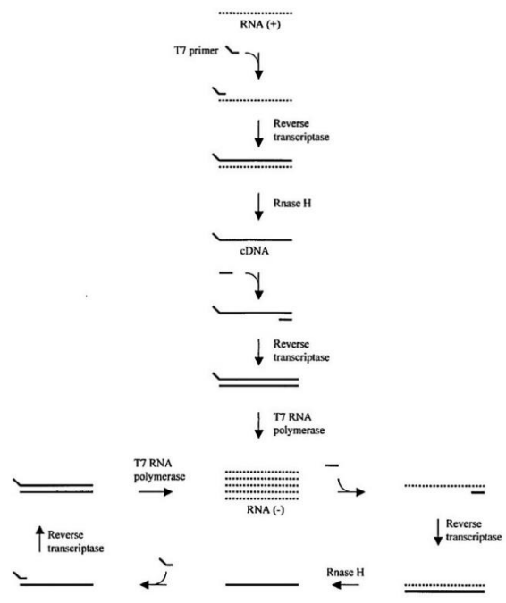
Figure 1. Schematic representation of the replication process in the NASBA technique
