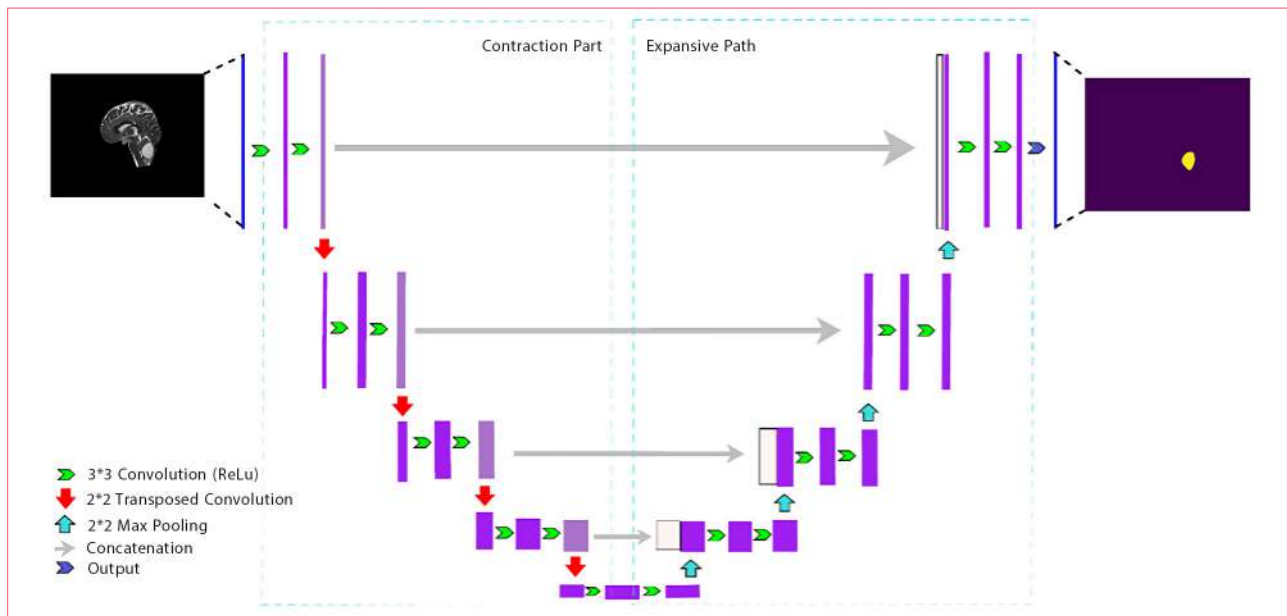
Figure 1. U-Net structure with 4 encoding and 4 decoding blocks
