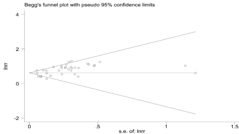
Fig.3: Begg's plot for publication bias of all studies ( P=0.256>0.5 )
