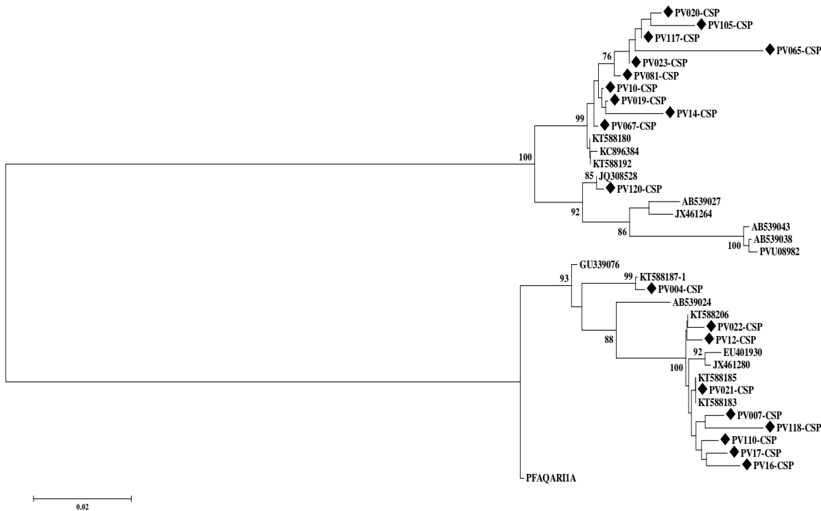
Fig. 3: Phylogenetic tree was drawn using Neighbor-Joining statistical method applying Kimura 2-parameter method for different strains of P. vivax parasite for CSP gene based on substitution changes in nucleic acid
