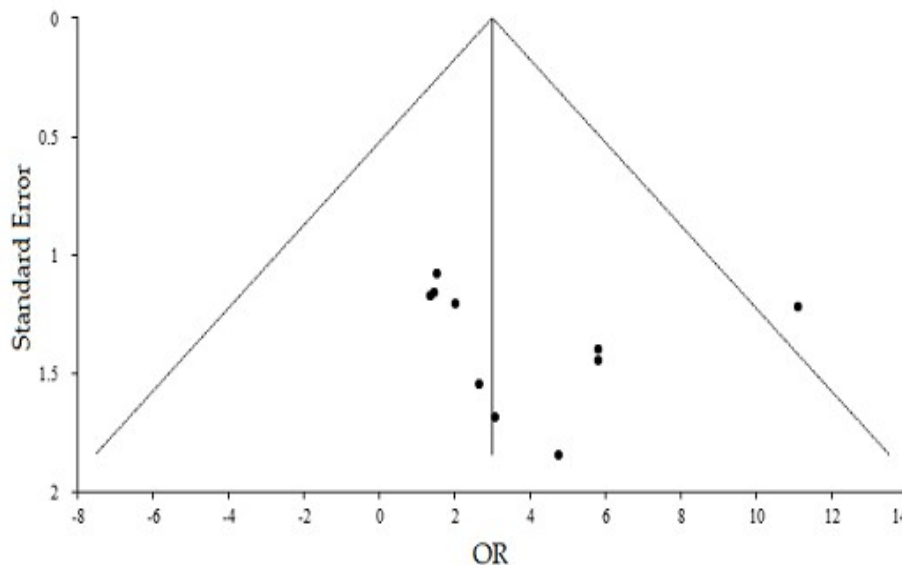
Fig. 3: Funnel Plot
