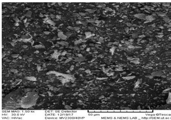
Fig. 3: SEM view of 1w group
