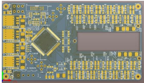
Figure 2. The LED driver as a 4-layer PCB designed in Altium designer
