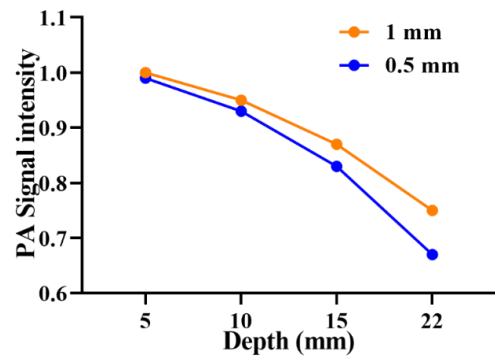
Figure 4. PA signal intensity in different depths for two different diameters of graphite
