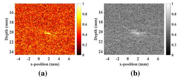
Figure 5. a) PA and b) Ultrasound image of object in depth 20 mm in agar phantom 1%
