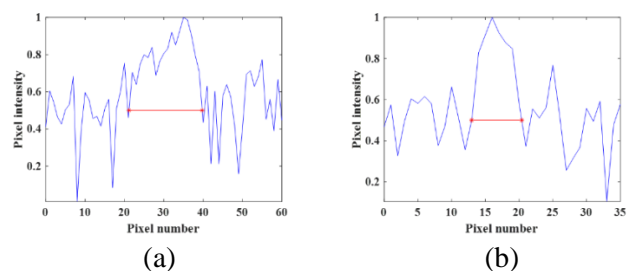
Figure 6. a) Lateral and b) Axial profile of needle photoacoustic image in depth 20 mm
