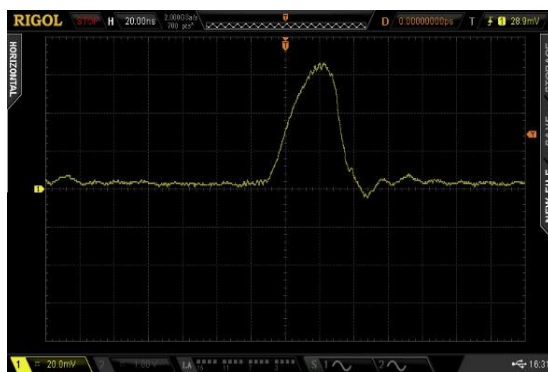
Figure 3. Optical pulse that is generated by high power LED mounted on driver board
