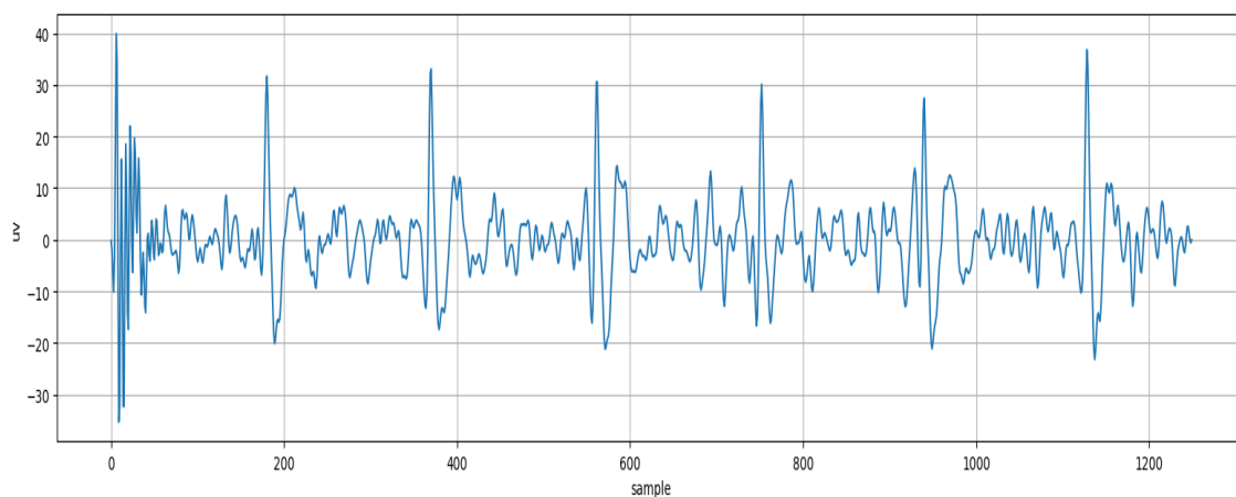
Figure 7. A small portion of time domain EEG signal for subject 8
