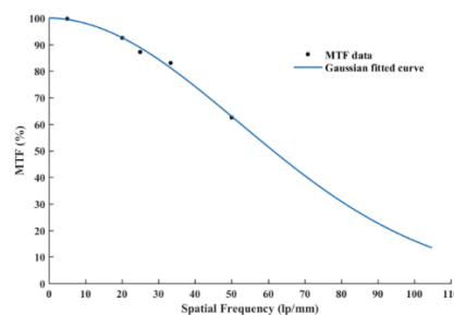
Figure 2. MTF curve acquired from bar phantom scanning by LOTUS-inVivo micro-CT. A Gaussian curve is fitted to MTF points
