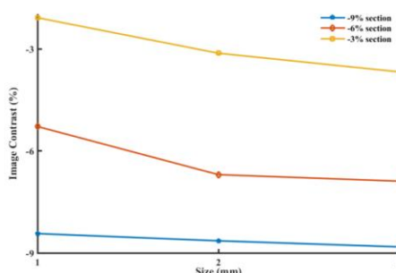
Figure 4. Image contrast of each phantom contrast section vs. the sizes available in LCD phantom (1, 2, and 3 mm) scanned by LOTUS-inVivo
