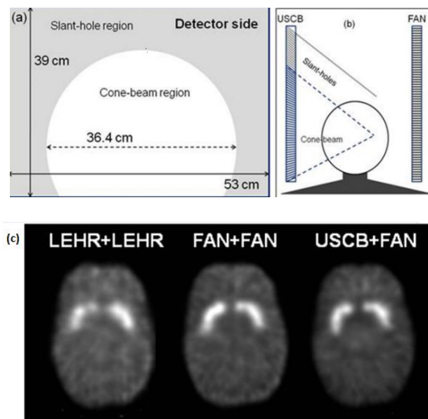
Figure 2. Schematic view of an Ultrashort Cone-Beam (USCB) collimator, (a) detector side of the collimator, (b) the collimator configuration for a brain SPECT acquisition combining USCB and FAN collimators, (c) Transverse slice through reconstructed images of the striatal phantom with a 5:1 striatal/background concentration of ^{99m}\text{Tc} [27]
