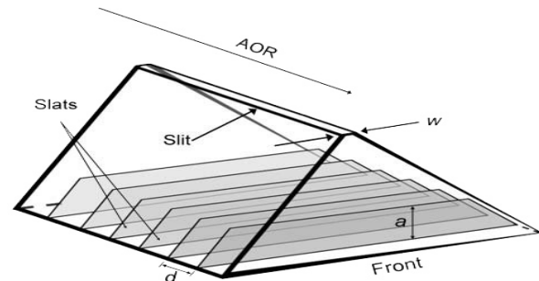
Figure 5. Schematic configuration of a slit-slat collimator. The slit is parallel to the Axis of Rotation (AOR). Normal to slats are also parallel to AOR. ( \alpha : slat height; d : slat spacing; and w : slit width) [6]
