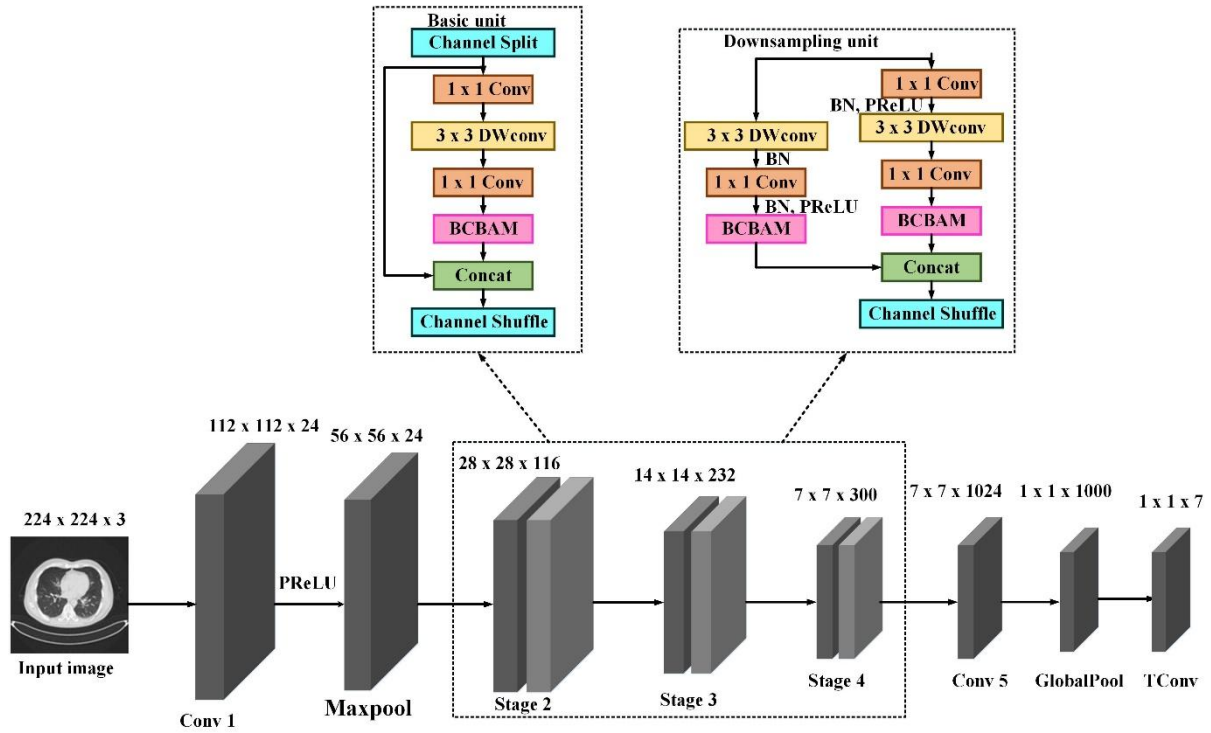
Figure 5. The structure of the Modified ShuffleNetV2 model
