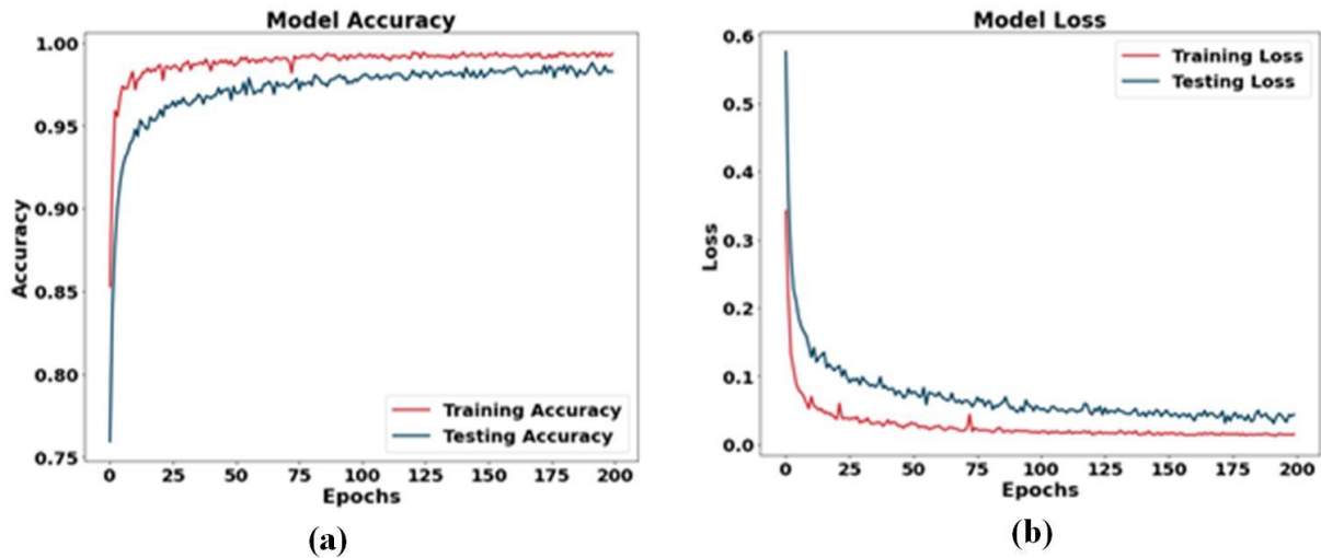
Figure 14. Accuracy and loss score graph for the training and testing sets for the LIDC-IDRI dataset
