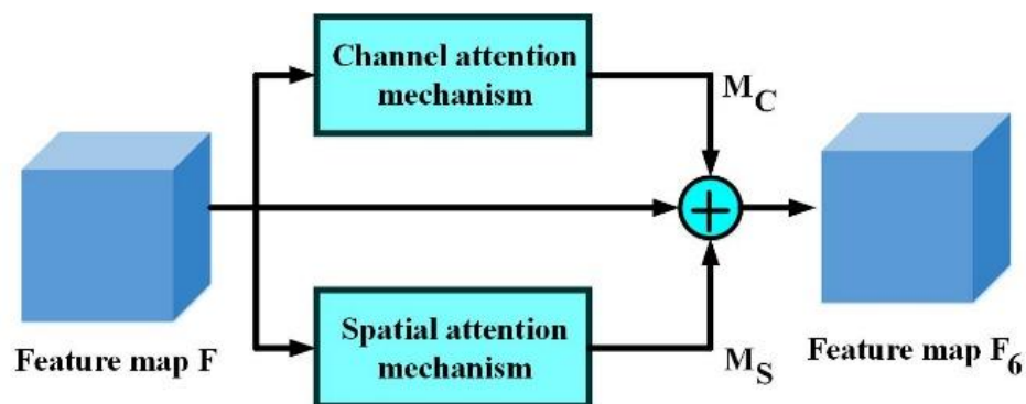
Figure 6. The structure of BCBAM
