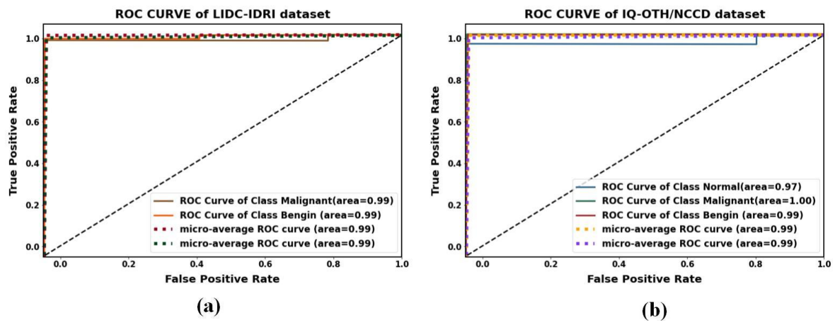
Figure 15. ROC curve for lung cancer classification using (a) LIDC-IDRI dataset and (b) IQ-OTH/NCCD dataset
