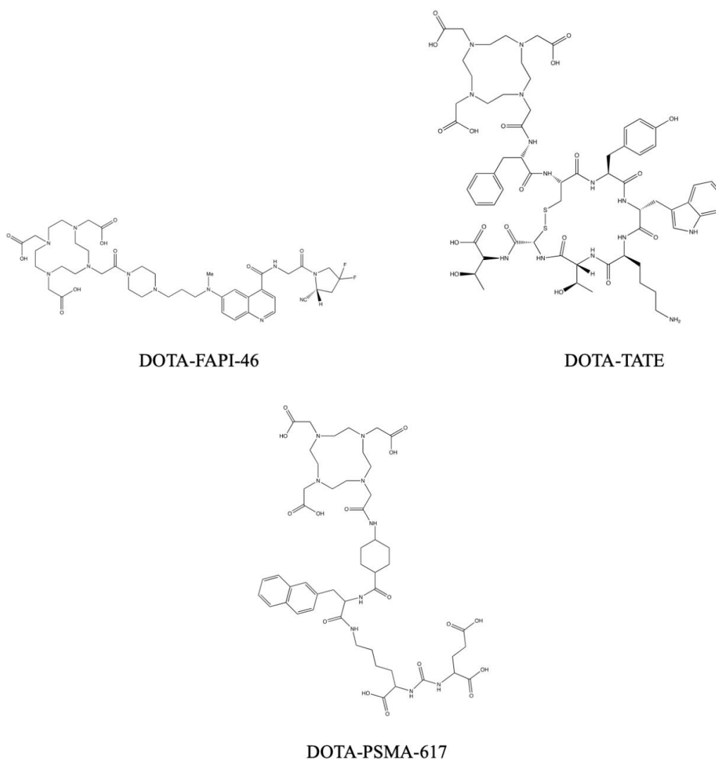
Figure 2. The chemical structure of DOTA-TATE, PSMA-617, and FAPI-46
