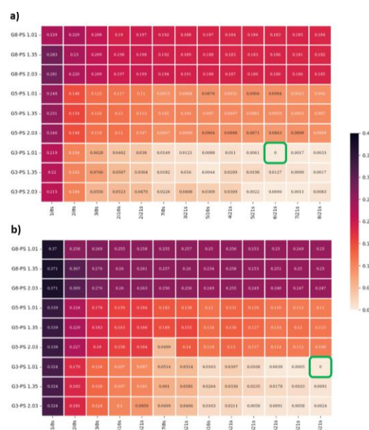
Figure 4. The relative difference percentage value of SUV_{max} in various image reconstruction sets in (a) non-RR OSEM3D image reconstructions with the green box as the reference (6i21s, 3 mm FWHM and pixel size= 1.01 mm), (b) RR OSEM3D image reconstructions with the green box as the reference (8i21s, 3 mm FWHM and pixel size= 1.01 mm). GN: Gaussian filter with N mm FWHM. PS: pixel size (mm). All values are rounded to the nearest five percent
