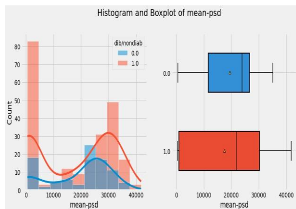
Figure 11. Histogram and Boxplot of mean-Psd
