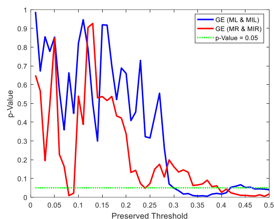
Figure 7. Evaluation of the difference in the distribution of GE values of the main graph in two classes of ML-MIL and MR-MIR using t-test analysis
