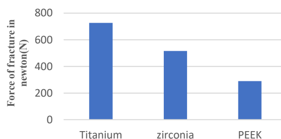
Figure 5. The force required for the fracture of the three abutment materials
