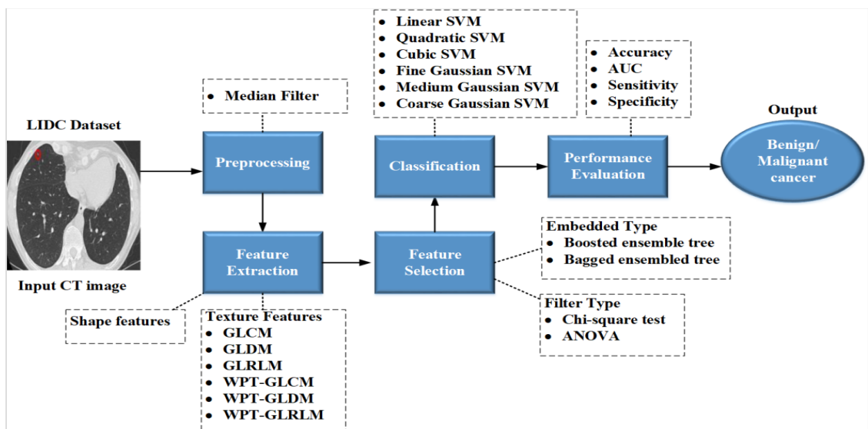
Figure 2. Proposed framework to diagnose lung cancer
