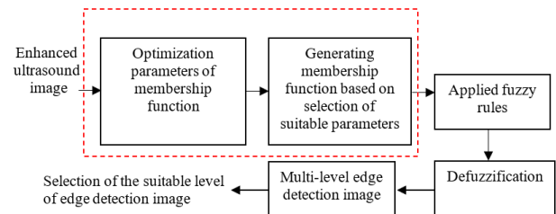
Figure 3. Fuzzy edge detection step [19]
