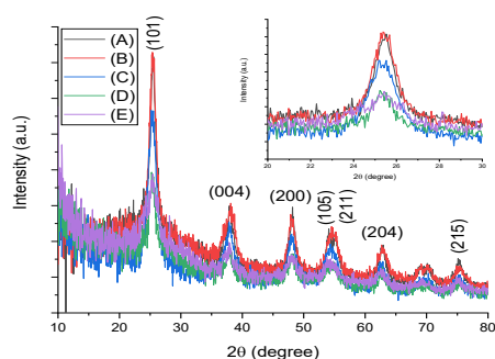
Figure 3. XRD of (a) \text{TiO}_2 , (b-d) 1,5 and 10wt.% rGO/Cu- \text{TiO}_2
