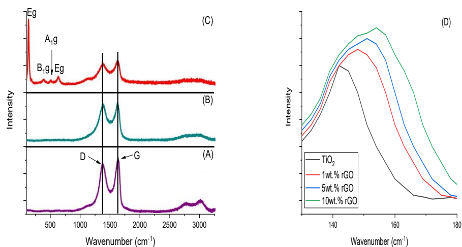
Figure 5. Raman spectrum of (a) GO, (b) rGO, (c) 5wt.% rGO/Cu-TiO 2 , and (d) Eg peak intensity of TiO 2
