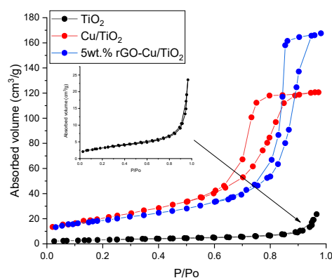
Figure 10. BET of bare, Cu, and 5wt.%r GO/Cu-TiO 2
