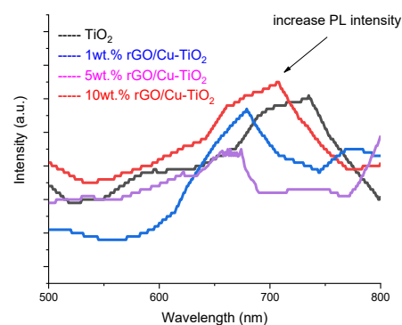
Figure 9. PL spectrum of pure and wt.% rGO/Cu-TiO 2 nanocomposite
