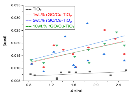
Figure 4. Williamson-Hall plot of pure and wt.% rGO/Cu-TiO 2
