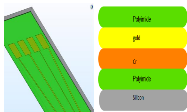
Figure 3. Structure of design A [6]
