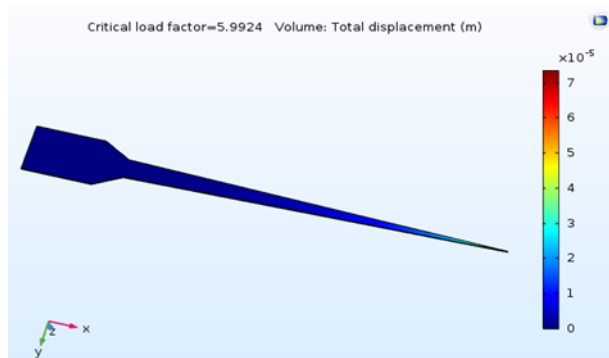
Figure 15. Displacement of design C
