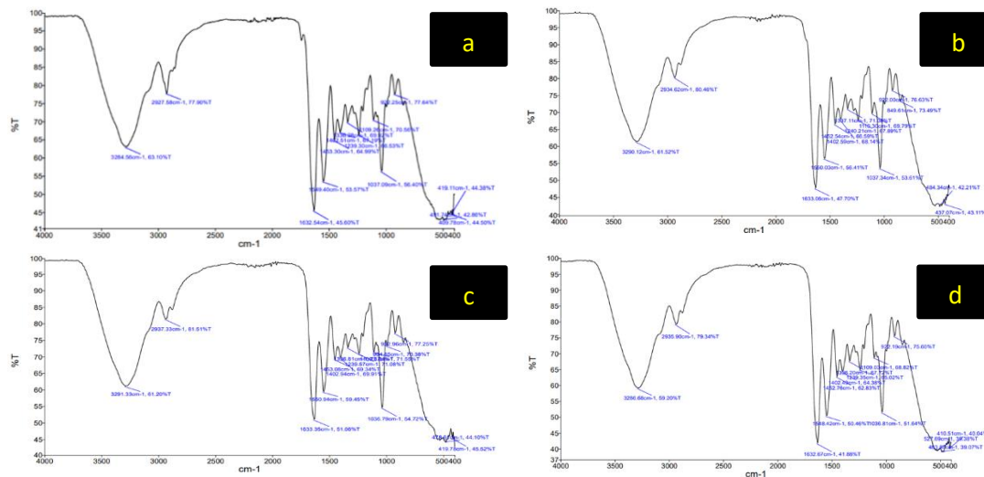
Figure 1. FTIR of whey-gelatin edible film with incorporation of (a) cinnamon essential oil; (b) clove essential oil; (c) basil essential oil; (d) lemongrass essential oil.
