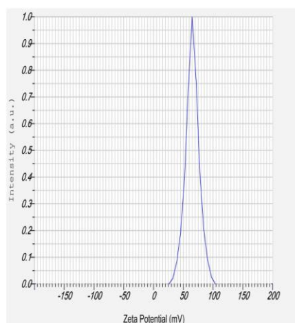
Figure 4. Zeta potential of Fe 3 O 4 nanoparticles containing quercetin.
