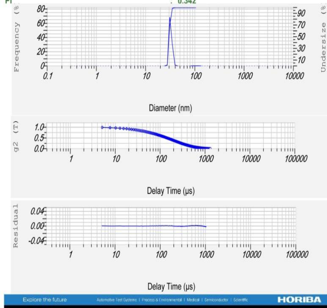
Figure 3. Size of Fe 3 O 4 nanoparticles containing quercetin drug.
