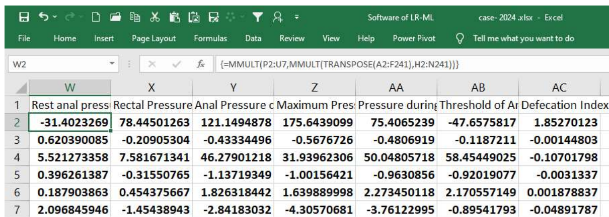
Figure 4. Hidden layer calculation using matrix multiplication: MMULT (P2:U7, MMULT [TRANSPOSE [A2:F241], H2:N241])
