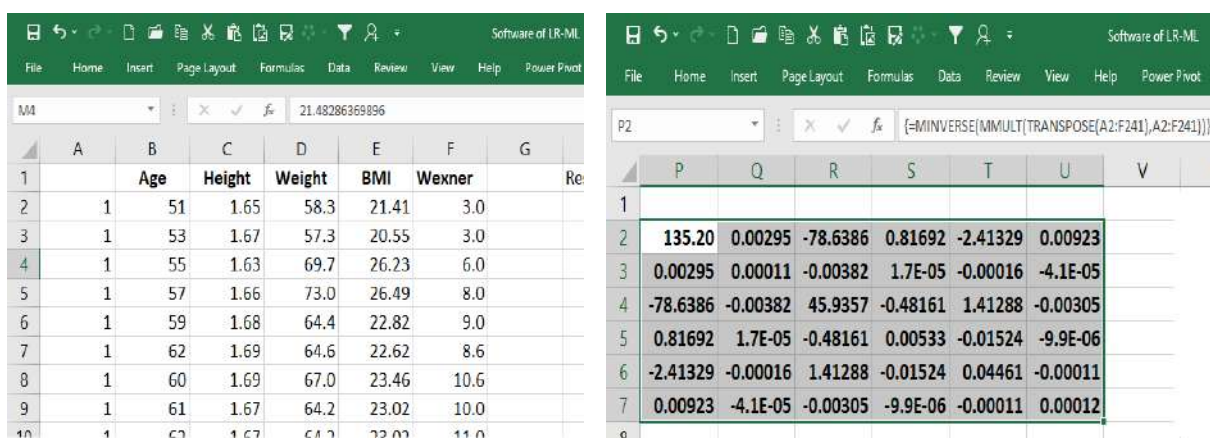
Figure 3. Input layer variables (age, height, weight, BMI, Wexner) and NMF equation (MINVERSE [MMULT [TRANSPOSE [A2:F241], A2:F241]]) in Excel
