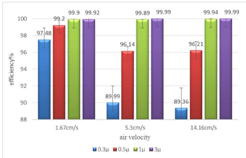
Fig. 5: Efficiency of particle removal of 0.3, 0.5, 1 and 3 \mu\text{m} size at three air flow velocity levels at 75% humidity by PDLLA polymer media
