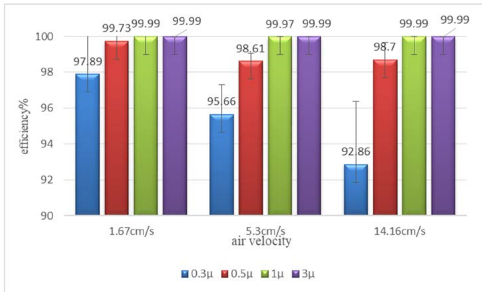
Fig. 4: Efficiency of particle removal of 0.3, 0.5, 1 and 3 \mu\text{m} size at three air flow velocity levels at 55% humidity by PDLLA polymer media
