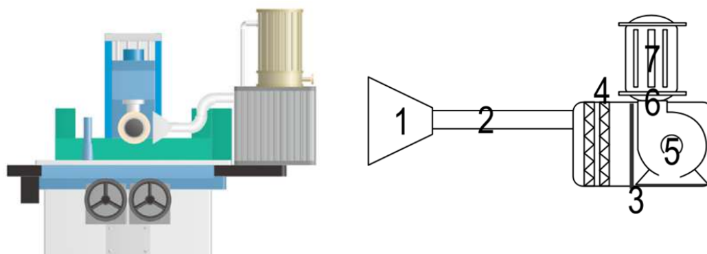
Fig. 1: Schematic of the designed local exhaust ventilation system (1 - Local extraction hood, 2 - Flexible accordion duct, 3 - Filtration chamber, 4 - Aluminum filter, 5 - Centrifugal fan with radial blades, 6 - Tube sheet, and 7 - Cartridge filter containing a metal-organic framework nanofiber)
