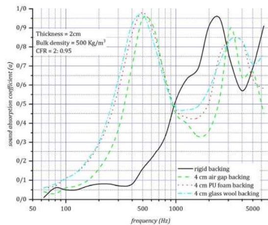
Fig. 2: Effect of backing layer on sound absorption of selected WWCP samples
