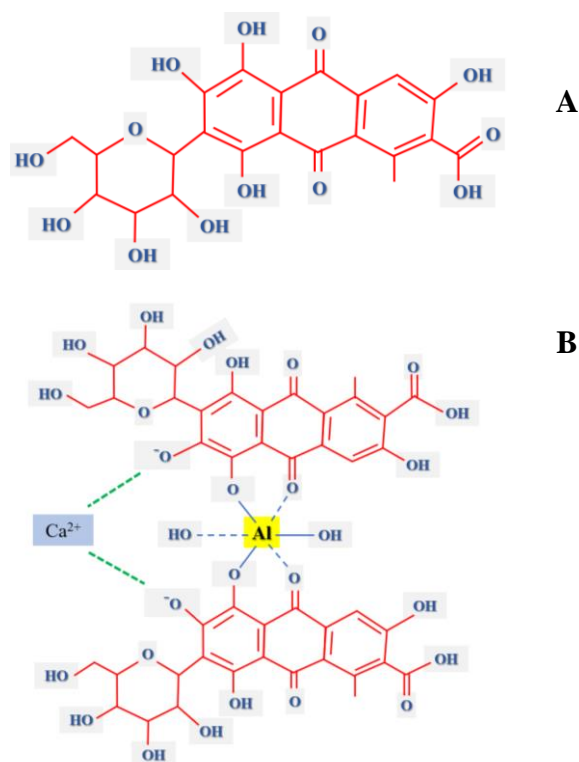
Figure 1: Chemical structure of A) carminic acid; B) aluminum lake of carmine combined with calcium (Ca 2+ )
