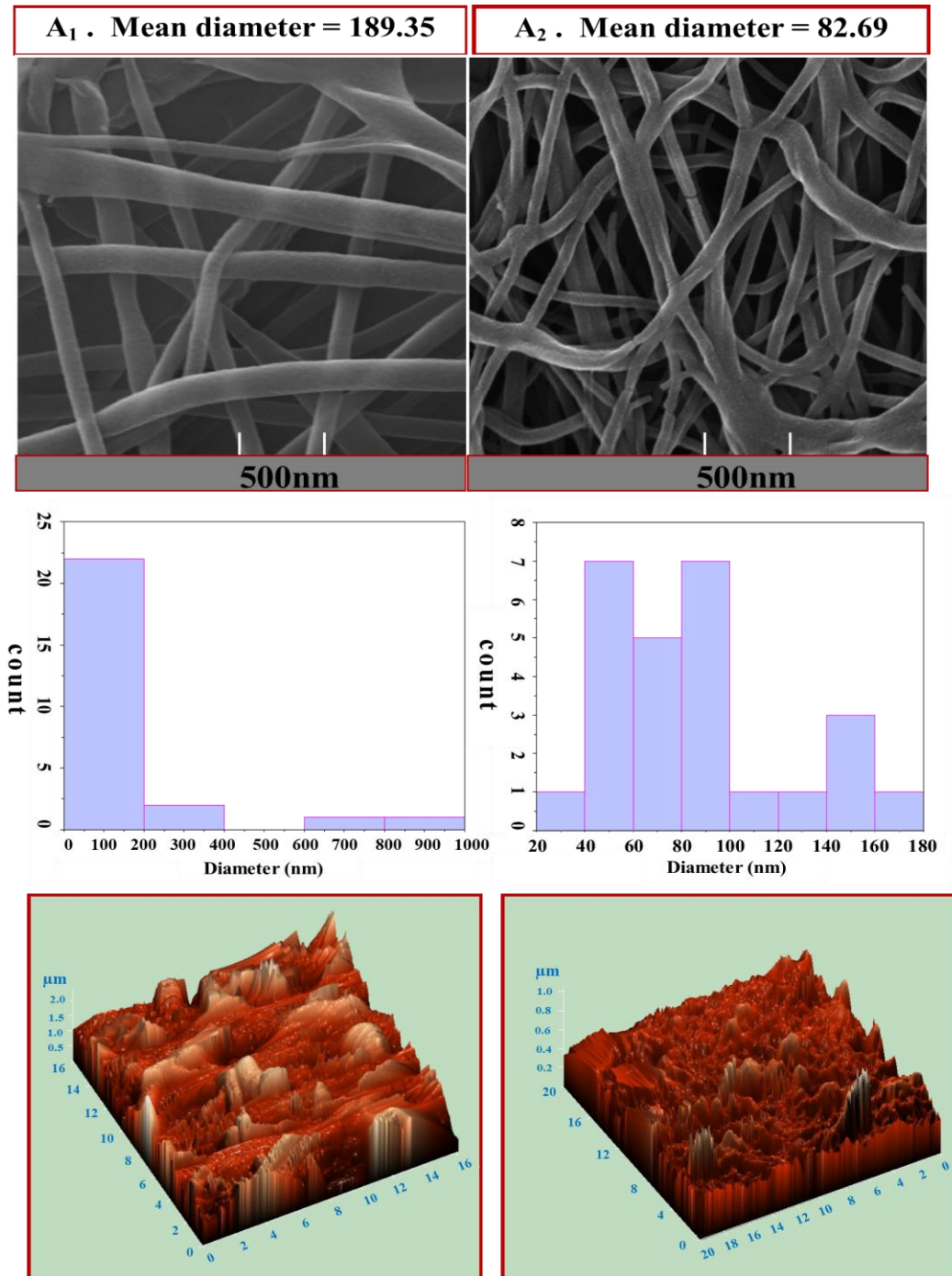
Figure 2: Field Emission-Scanning Electron Microscopy (FE-SEM) micrographs, diameter distribution histograms, and Atomic Force Microscope (AFM) of the electrospun nanofibers. A 1 : PCL; A 2 : PCL 90%+BSG 10% BSG=Basil Seed Gum; PCL=Polycaprolactone
