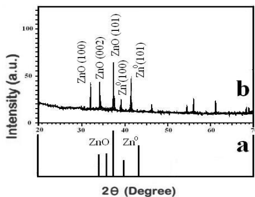
Figure 2: Standard Zn-ZnO powder diffraction pattern (a) and XRD pattern of nano nZ 0 -ZnO
