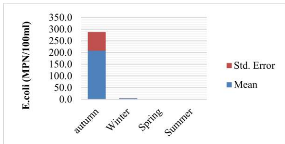
Figure 2: Seasonal variation of physicochemical parameters and indicator of bacteria
