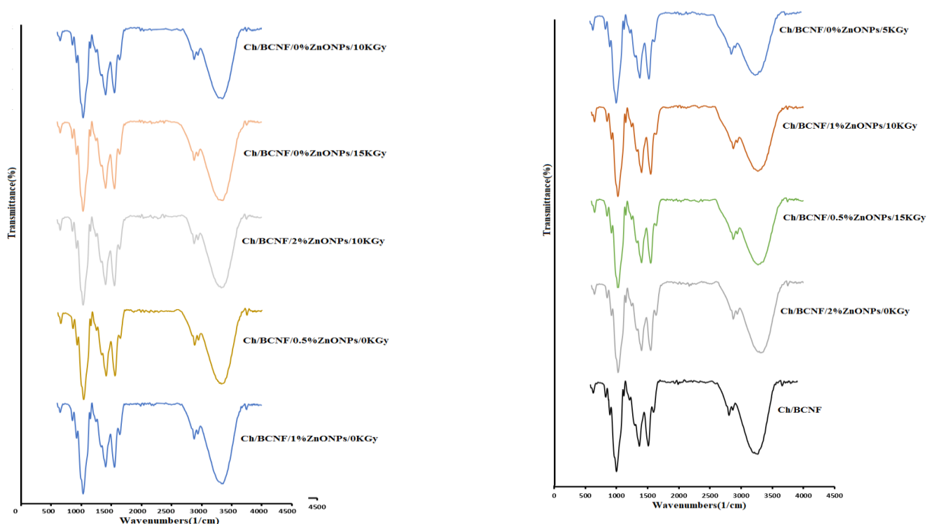
Figure 4: ATR-FTIR spectra of different types of non-irradiated and irradiated Ch/BCNF films (in color).
