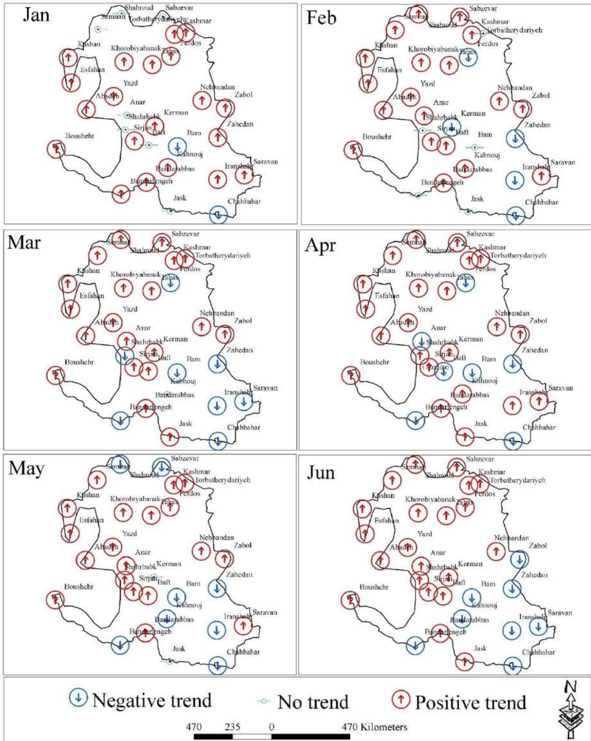
Figure 4: Mann-Kendall statistics values related to monthly changes of external-origin dust in arid cities of Iran
