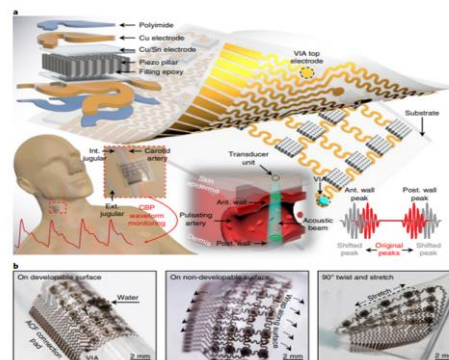
Figure 9. Design and mechanism of the tensile ultrasound machine
