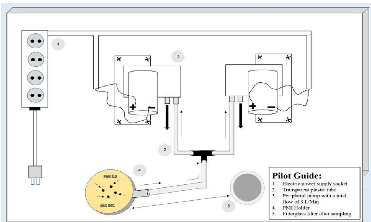
Fig. 2. Sampling pilot's schematic
