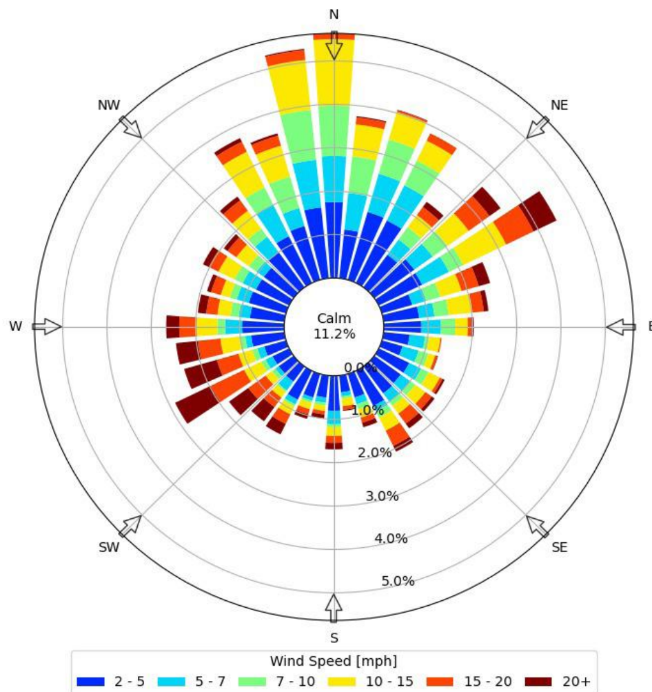
Fig. 7. wind rose in Arak city (2017-2020)
