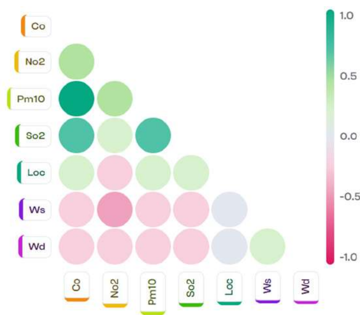
Fig. 14. Correlation between variables determining air pollution
