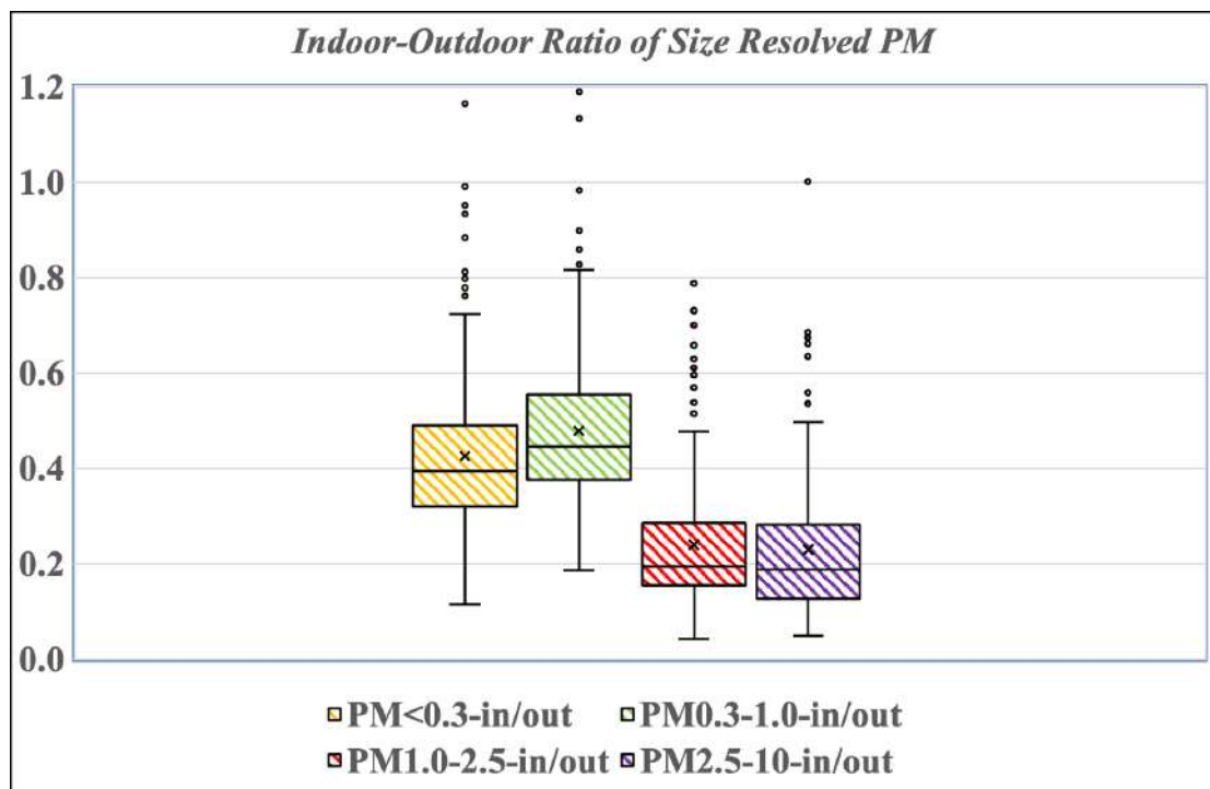
Fig. 5. Box plot for a) indoor-outdoor, b) I/O distribution of size-fractionated ( PM_{10} , PM_{2.5} , PM_{1.0} , and PM_{0.3} ), c) I/O distribution of size-resolved ( PM_{2.5-10} , PM_{1.0-2.5} , PM_{0.3-1} and PM_{<0.3} ) particles for site B
