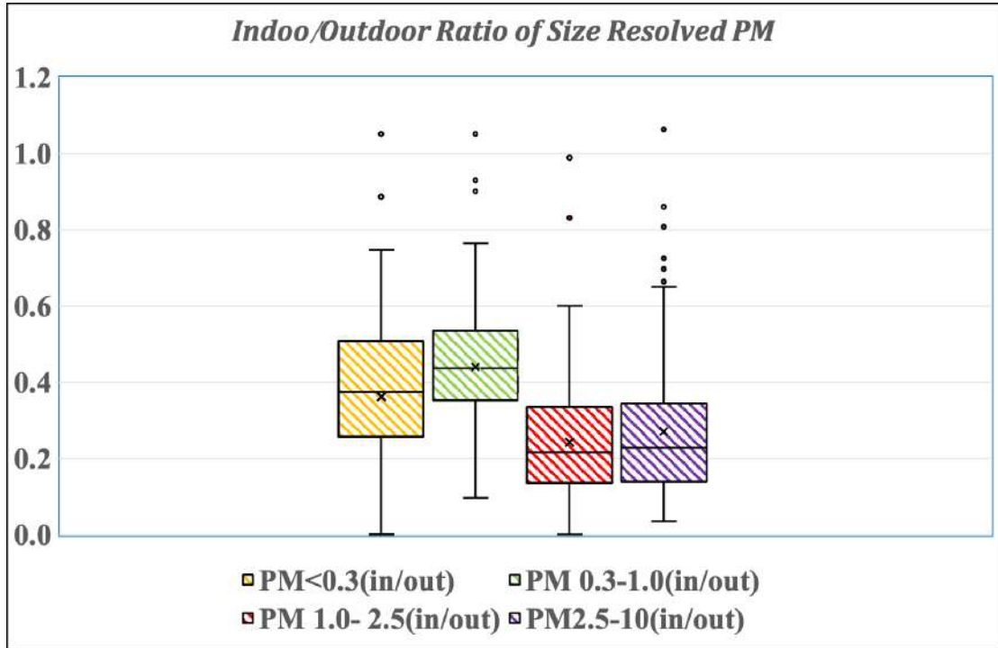
Fig. 4. Box plot for a) indoor-outdoor, b) I/O distribution of size-fractionated ( PM_{10} , PM_{2.5} , PM_{1.0} , and PM_{0.3} ), c) I/O distribution of size-resolved ( PM_{2.5-10} , PM_{1.0-2.5} , PM_{0.3-1} and PM_{<0.3} ) particles for site A
