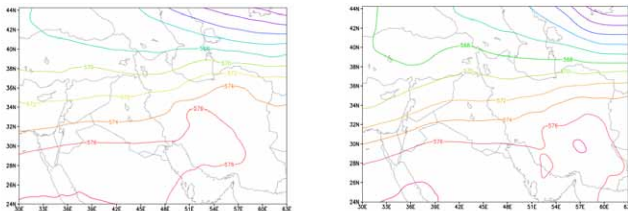
Fig. 12. Shows geopotential elevation of the level 500 hPa (gpm) at 12UTC on day: a) 2 nd July; (b) 3 th July 2016)
