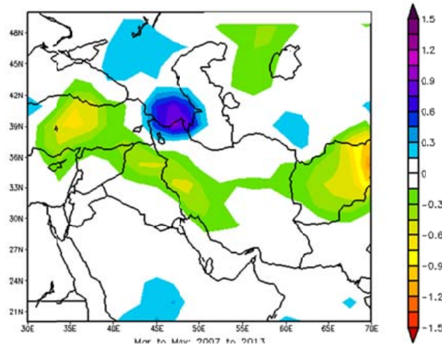
Fig. 4. The spring precipitation anomaly from 2007 to 2013 relative to the annual average for the period 30-years (1981 to 2010)
