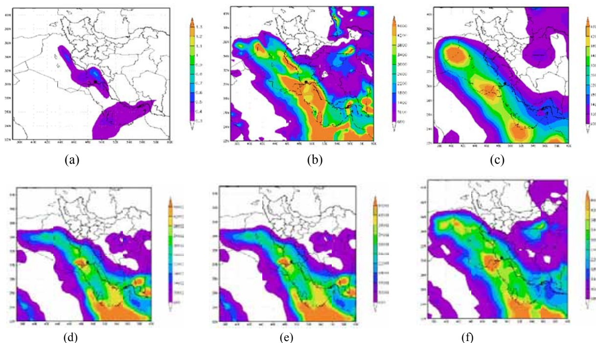
Fig. 14. The dust concentration in 4 July 2016, 18UTC for (a) MACC-ECMWF (b) NASA-GEOS (c) NCEP-NGAC (d) NMMB-BSC (e) DREAM-BSC (f) the mean of all the models
