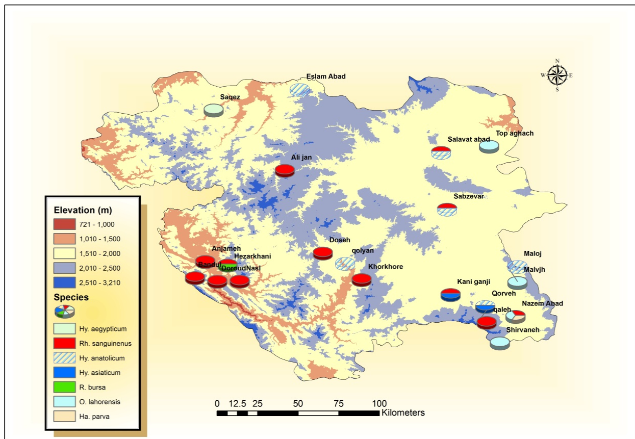
Fig. 2. Spatial distribution of livestock ticks in different altitudinal categories of Kurdistan Province of Iran, 2012-2013
