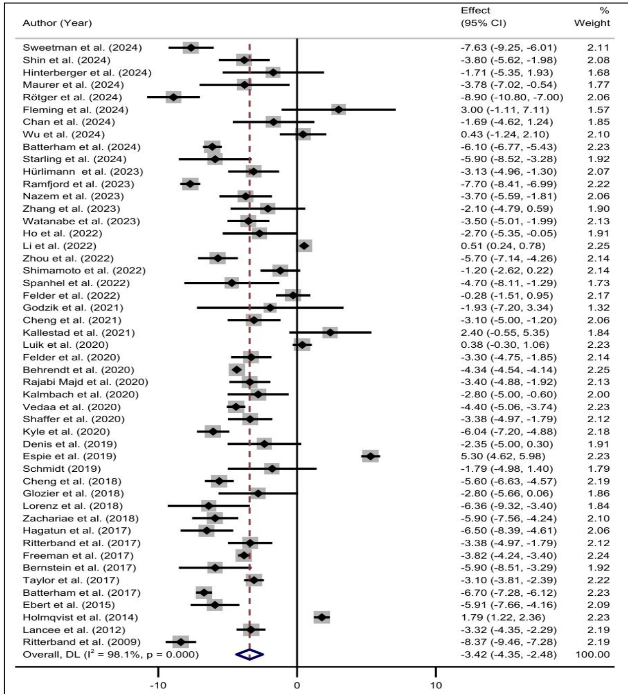
Figure 2. Forest Plot The Effectiveness of Fully Automated Digital Cognitive Behavioral Therapy for Insomnia, Expressed as the Mean Differences between the Intervention and the Control Groups
