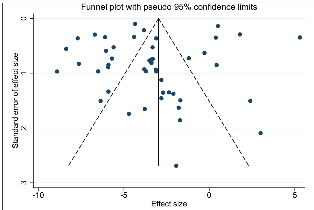
Figure 3. Funnel Plot for Assessing Publication Bias in Meta-Analysis of Fully Automated Digital Cognitive Behavioral Therapy for Insomnia
