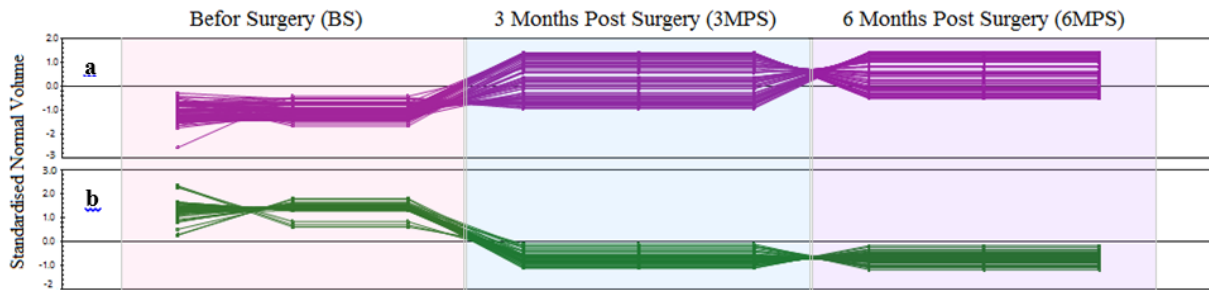
Fig. 2: Expression patterns of (a) increased and (b) decreased proteins in three groups of patients including BS (Before Surgery), 3MPS (3 Months Post-Surgery) and c) 6MPS (6 Months Post-Surgery). Diagram was obtained from Progenesis SameSpots software
