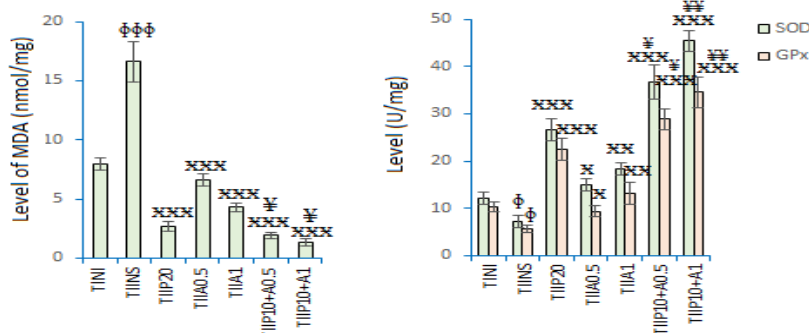
Fig. 2: Effects of AuNPs and PYR on tissue MDA levels and GPx and SOD enzyme activity in dexamethasone-immunosuppressed, T. gondii -infected mice. Data are expressed as mean \pm SD (N=8). \phi P<0.05 , \phi\phi\phi P<0.001 vs. TINI; \times P<0.05 , \times\times P<0.01 , \times\times\times P<0.001 vs. TIINS; \yen P<0.05 vs. TIIP20
