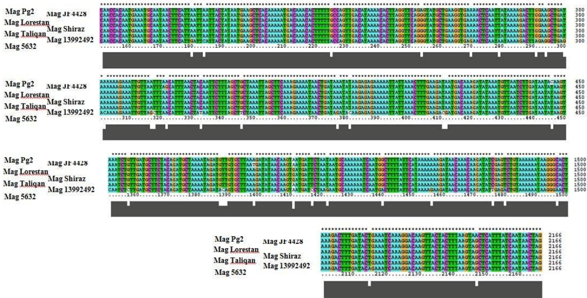
Fig. 2. Genetic diversity at ma-mp81 gene between the three Iranian vaccine and four laboratory strains of Mycoplasma agalctiae PG2, 5632, JF4428 and 13992492 as viewed by Clustal W. Asterisks depict identical matches of nucleotides. Numbers indicate nucleotide positions within the 2, 166 nucleotide-long ma-mp81 gene.
