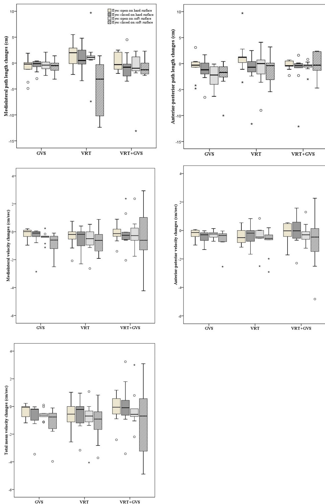
Figure 1. Median, minimum, and maximum changes of mediolateral and anterior-posterior path length and velocity, and total mean velocity of the center of pressure in four conditions in three groups. GVS; galvanic vestibular stimulation, VRT; vestibular rehabilitation therapy
