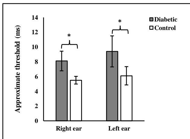
Fig. 1. Mean approximate threshold (milliseconds) in diabetic and control groups, * p < 0.05 .
