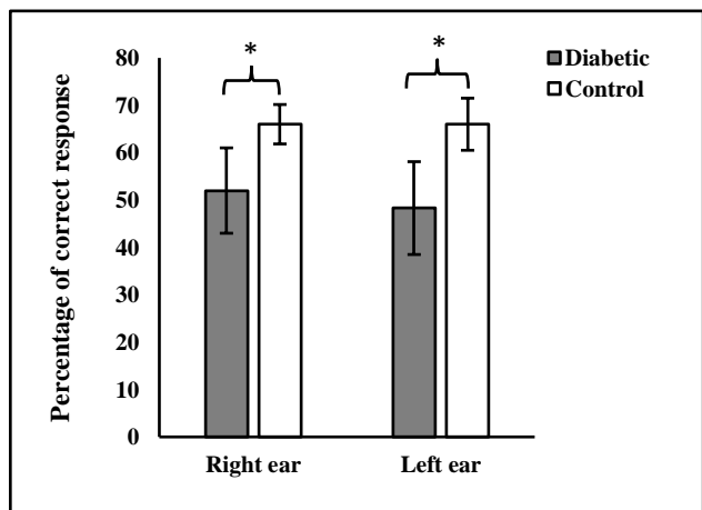
Fig. 2. Mean percentage of correct response in diabetic and control groups, *p<0.05.
