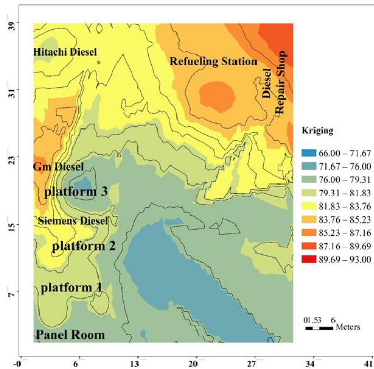
Figure 1. Isosonic map of the department and unite of Mashhad railway station.
