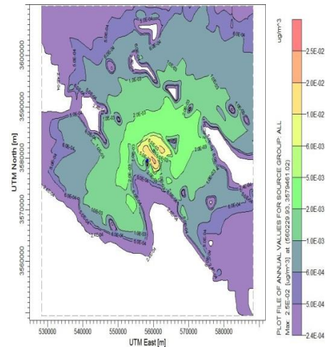
Figure 6. Annual average concentrations using AERMOD
