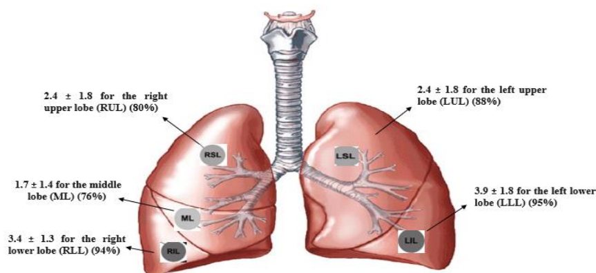
Figure 3. Lobar CT scores of patients Covid-19, data are expressed as mean value \pm SD (% of occurrences of involvement for each lobe) (*** P < 0.0001 ). RUL, right upper lobe; ML, middle lobe; RLL, right lower lobe; LUL, left upper lobe; LLL, left lower lobe
